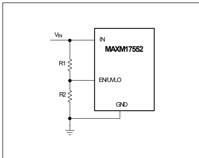
Figure 2. Adjustable EN/UVLO Network
