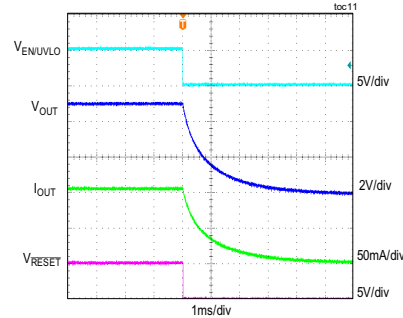
SHUTDOWN FROM EN/UVLO (5V OUTPUT, 100mA LOAD CURRENT, PWM MODE)
