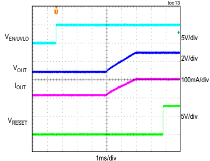
SOFT-START WITH 3V PREBIAS (100mA LOAD CURRENT, 5V OUTPUT, PWM MODE)
