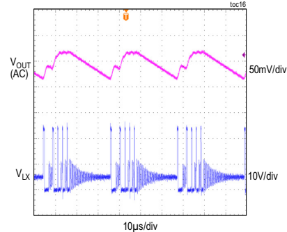
STEADY-STATE SWITCHING WAVEFORMS, (5V OUTPUT, 0.01A LOAD CURRENT, PFM MODE)
