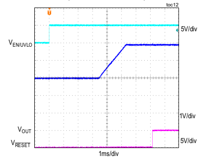
SOFT-START WITH 3V PREBIAS (5V OUTPUT, NO LOAD)
