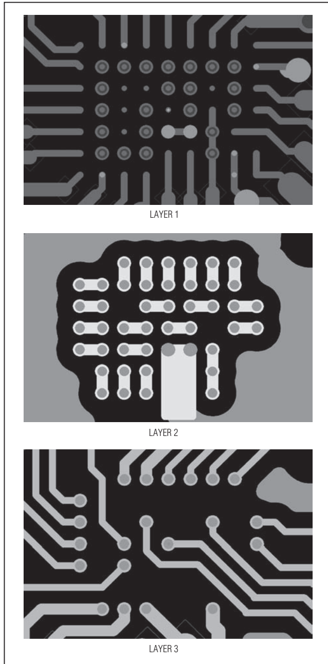
Figure 42. Suggested Routing
