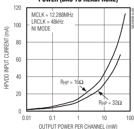
HPVDD INPUT CURRENT vs. OUTPUT POWER (DAC TO HEADPHONE)
