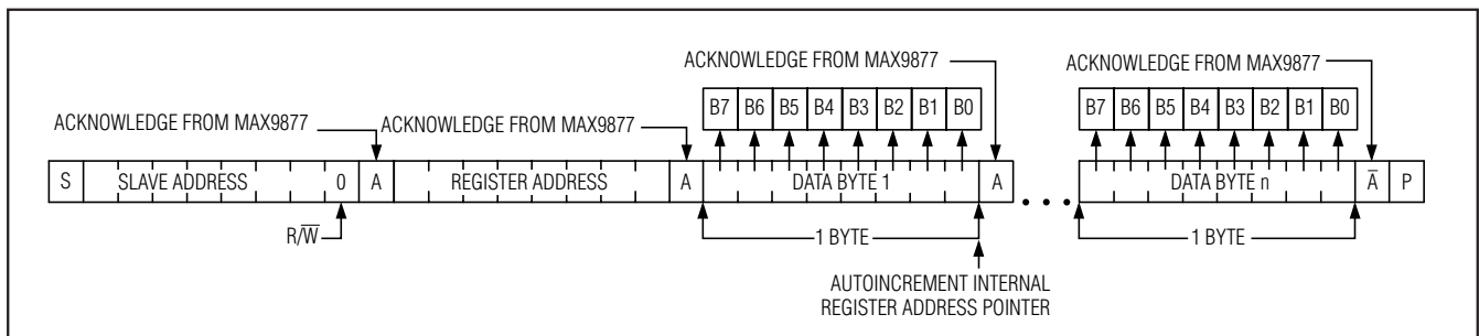
Figure 10. Writing n-Bytes of Data to the MAX9877
