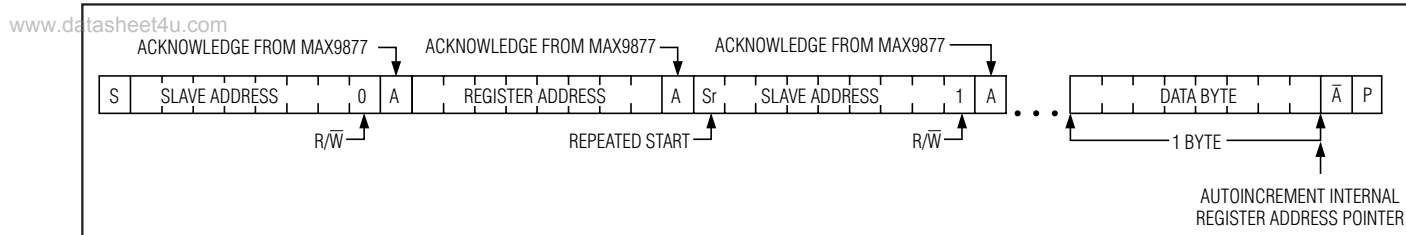
Figure 12. Reading n-Bytes of Indexed Data from the MAX9877
