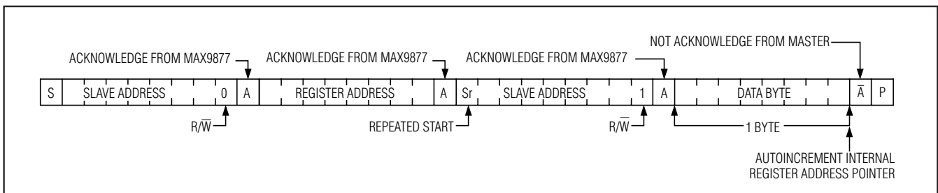
Figure 11. Reading One Indexed Byte of Data from the MAX9877
