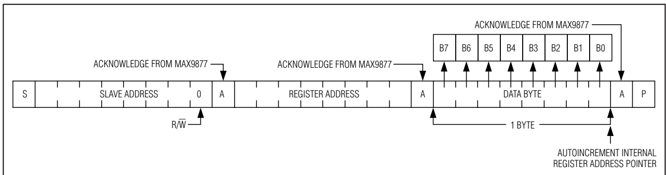
Figure 9. Writing One Byte of Data to the MAX9877
