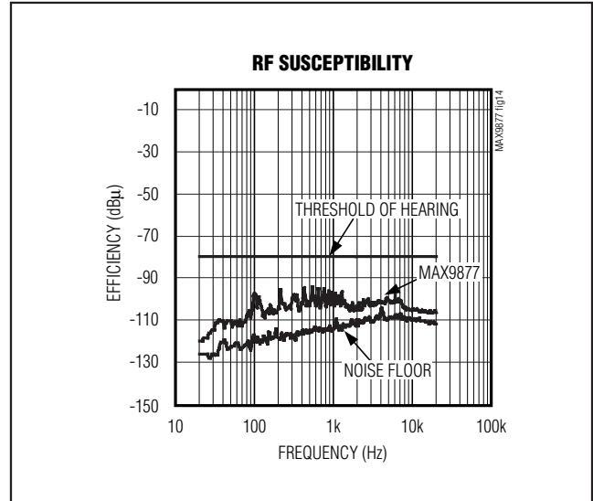
Figure 14. MAX9877 Susceptibility to a GSM Cell Phone Radio
