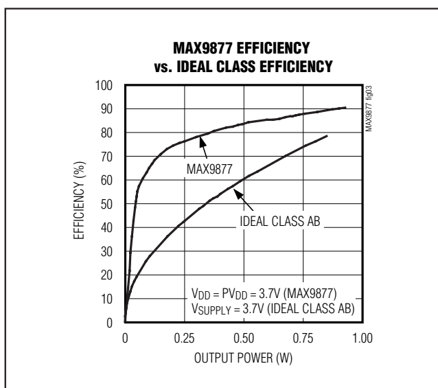
Figure 3. MAX9877 Efficiency vs. Class AB Efficiency
