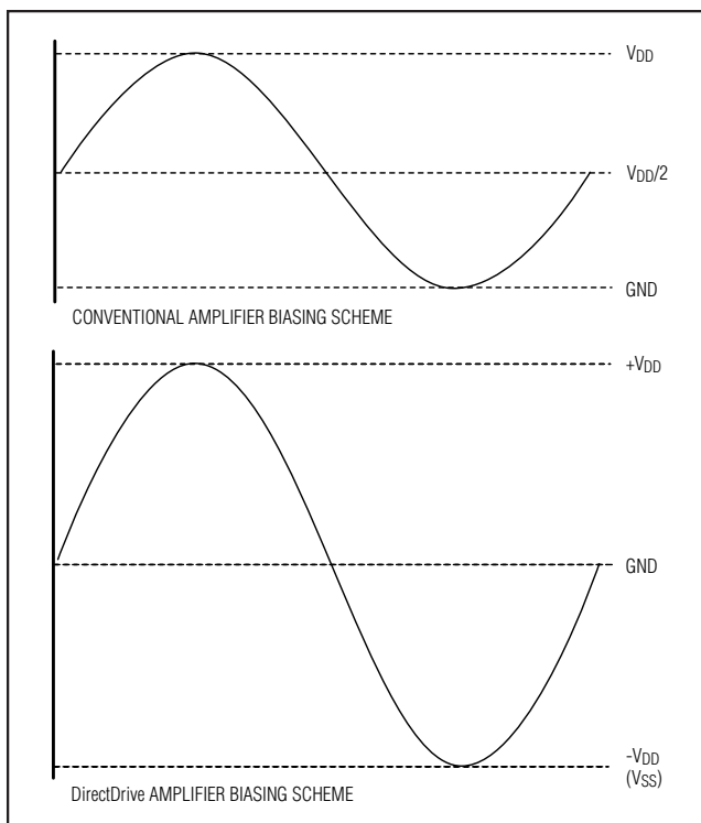
Figure 5. Traditional Amplifier Output vs. MAX9877 DirectDrive Output
