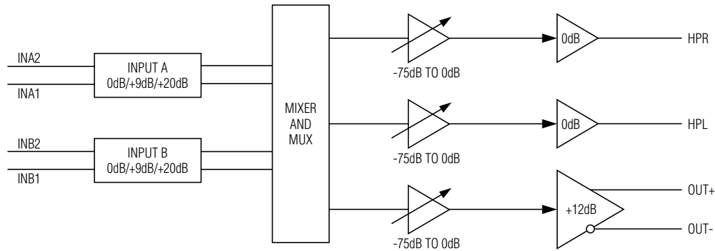
Figure 1. Signal Path
