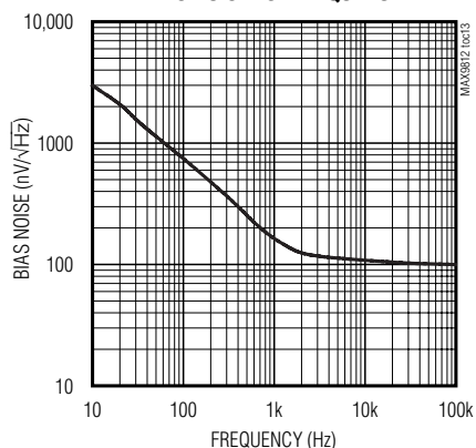
BIAS NOISE vs. FREQUENCY
