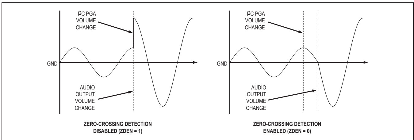
Figure 42. Zero-Crossing Detection
