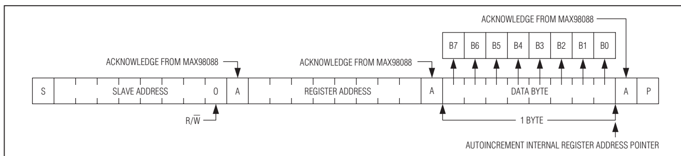
Figure 35. Writing One Byte of Data to the ICs
