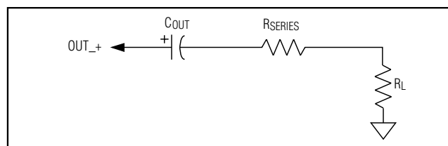
Figure 9. Reducing C_{OUT} by Adding R_{SERIES}
