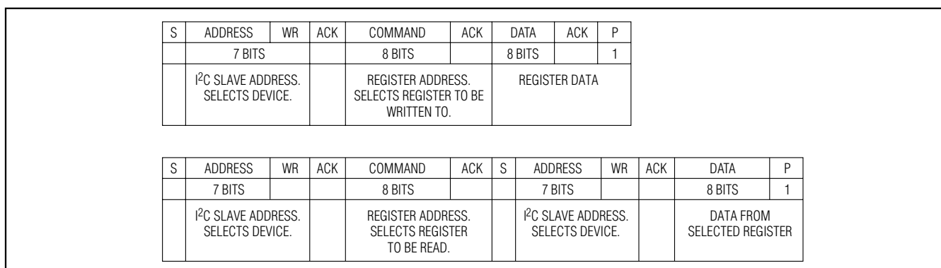
Figure 7. Write/Read Data Format Example
