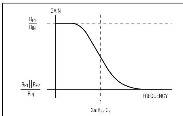
Figure 11. Bass Boost Response
