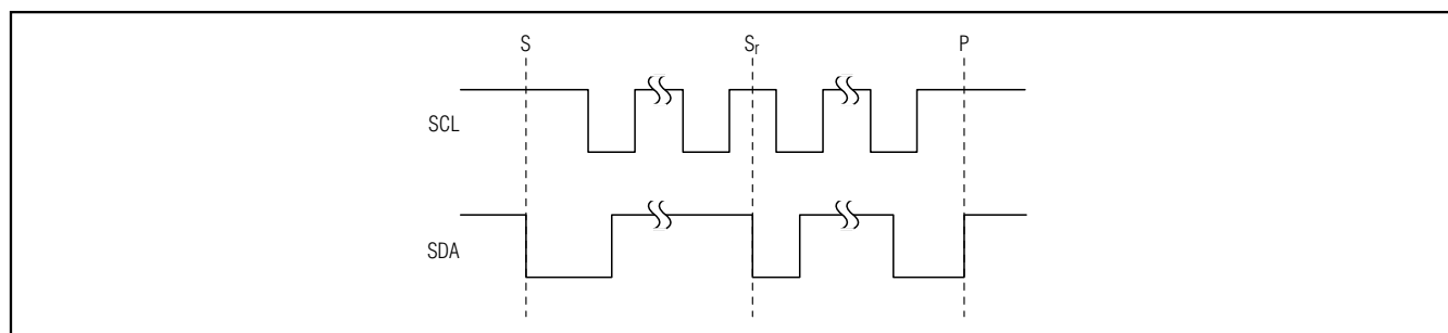
Figure 4. START/STOP Conditions
