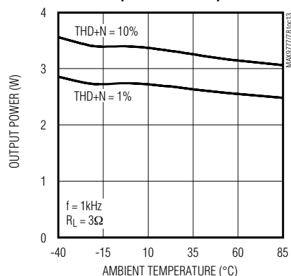
OUTPUT POWER vs. AMBIENT TEMPERATURE (SPEAKER MODE)
