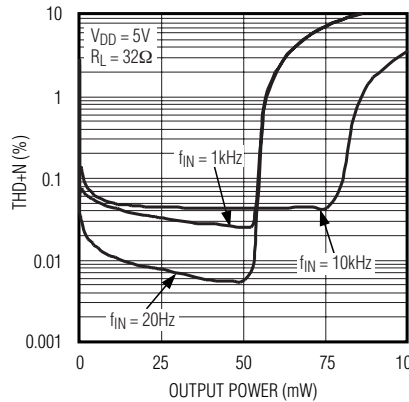
TOTAL HARMONIC DISTORTION PLUS NOISE vs. OUTPUT POWER (UCSP)
