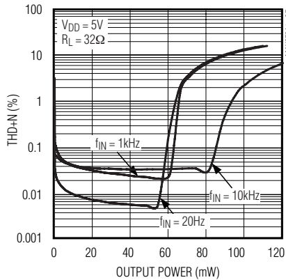
TOTAL HARMONIC DISTORTION PLUS NOISE vs. OUTPUT POWER (TQFN)
