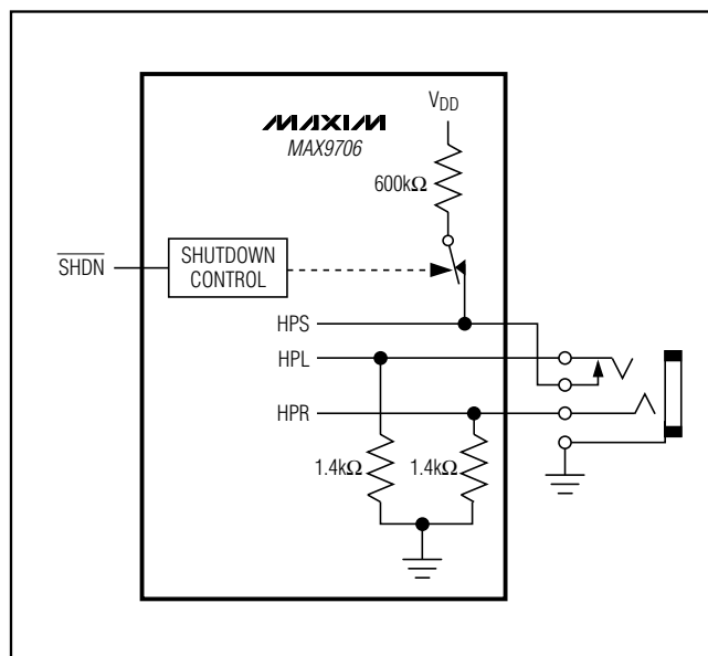
Figure 9. HPS Configuration
