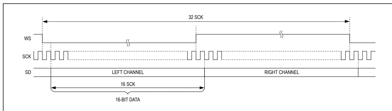
Figure 24. Stereo I 2 S (16-Bit Samples, No Padding)
