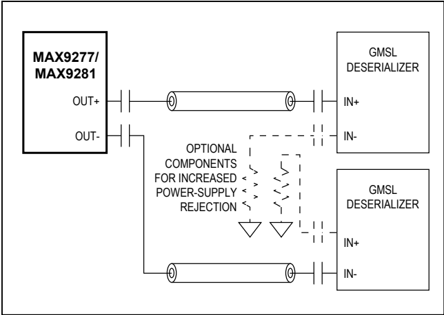
Figure 38. 2:1 Coax Splitter Connection Diagram
