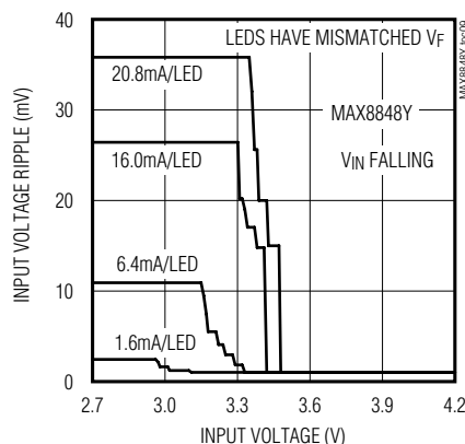
INPUT VOLTAGE RIPPLE (PEAK-TO-PEAK) vs. INPUT VOLTAGE
