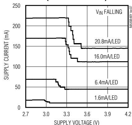
SUPPLY CURRENT vs. SUPPLY VOLTAGE (7 MISMATCHED LEDs)
