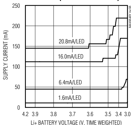
INPUT CURRENT vs. Li+ BATTERY VOLTAGE (7 MISMATCHED LEDs)
