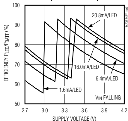
EFFICIENCY vs. Li+ BATTERY VOLTAGE (7 MISMATCHED LEDs)
