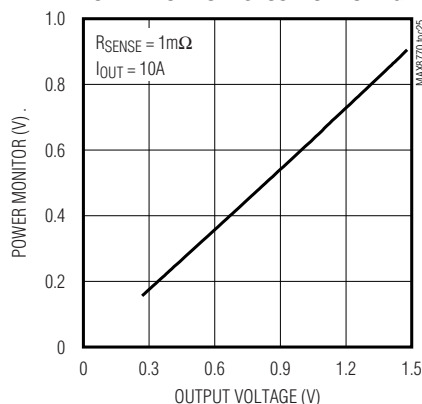
POWER MONITOR vs. OUTPUT VOLTAGE
