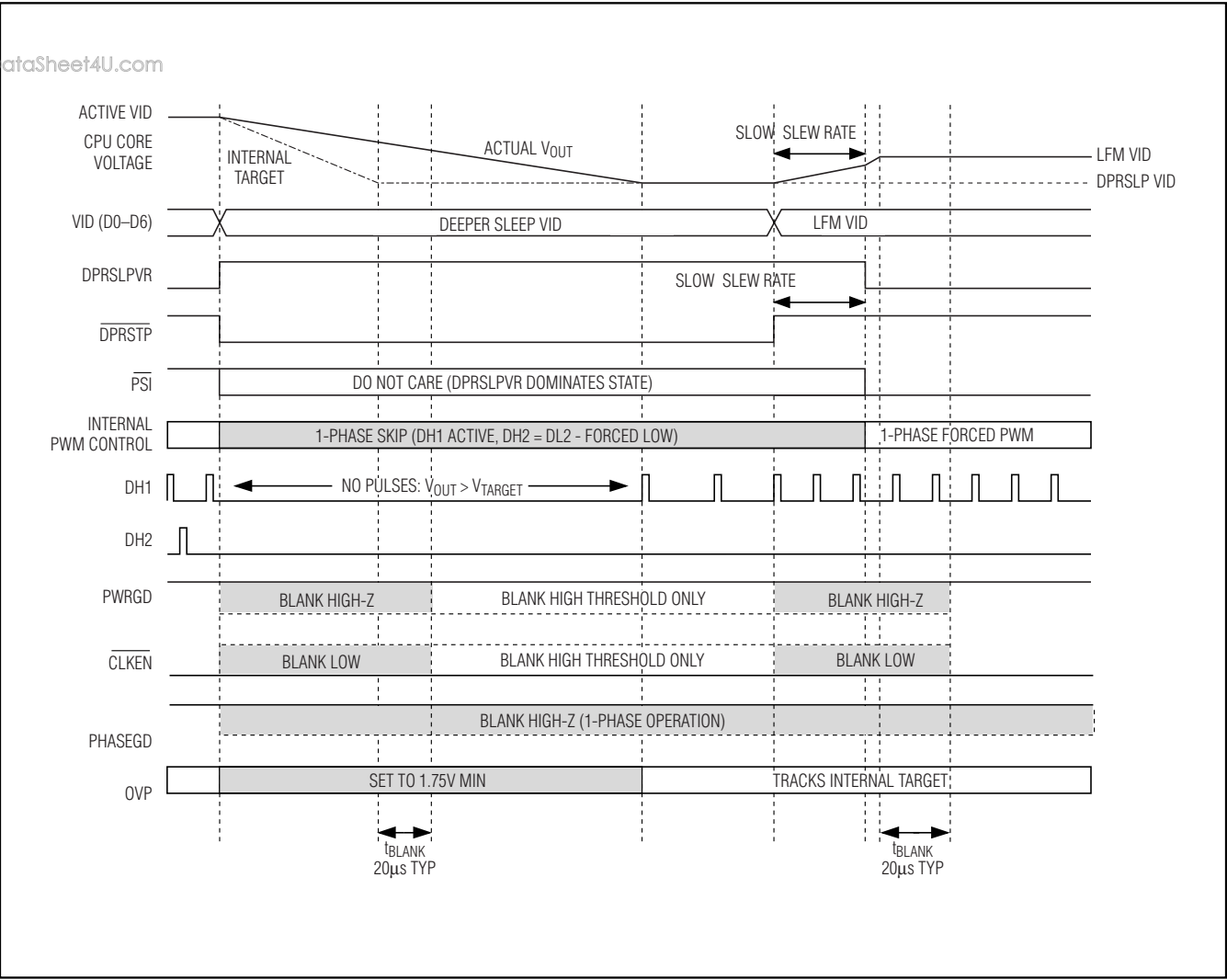
Figure 7. \overline{\text{PSI}} Transition
