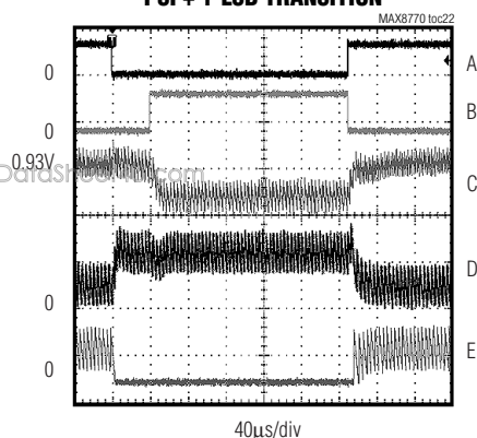
PSI + 1-LSB TRANSITION
