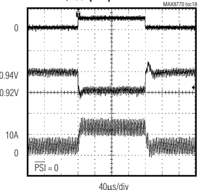
LFM LOAD TRANSIENT ( V_{OUT(LFM)} = 0.9500V )
