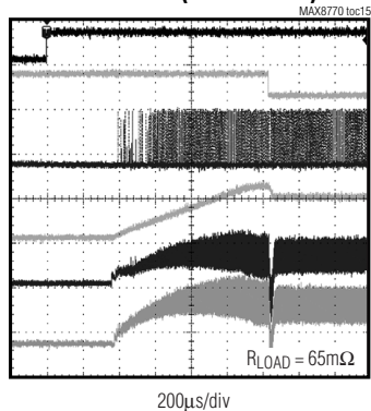
SOFT-START (UP TO CLKEN)
