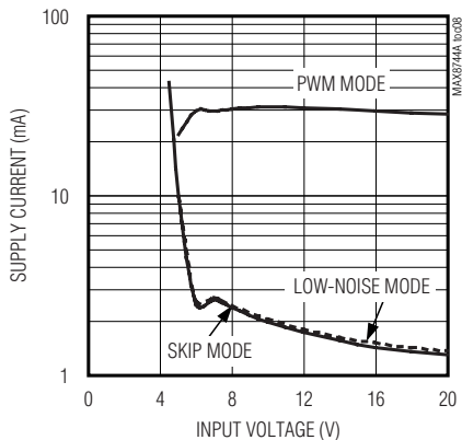
NO-LOAD INPUT SUPPLY CURRENT vs. INPUT VOLTAGE
