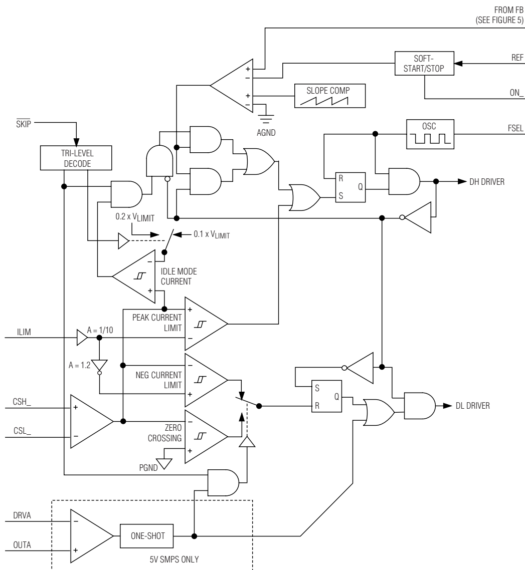
Figure 3. PWM Controller Functional Diagram
