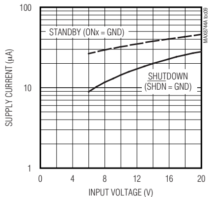
STANDBY AND SHUTDOWN INPUT CURRENT vs. INPUT VOLTAGE
