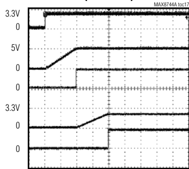
SMPS DELAYED STARTUP SEQUENCE (ON3 = REF)
