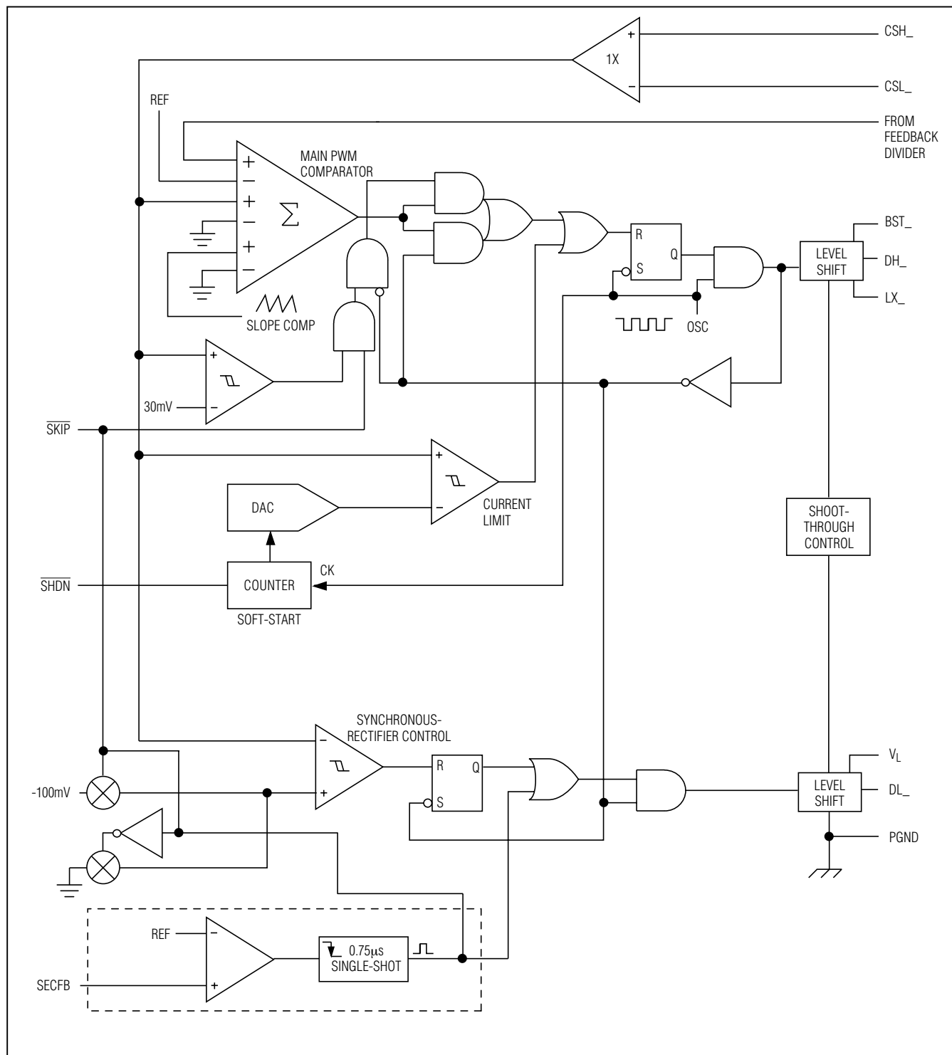
Figure 3. PWM Controller Functional Diagram
