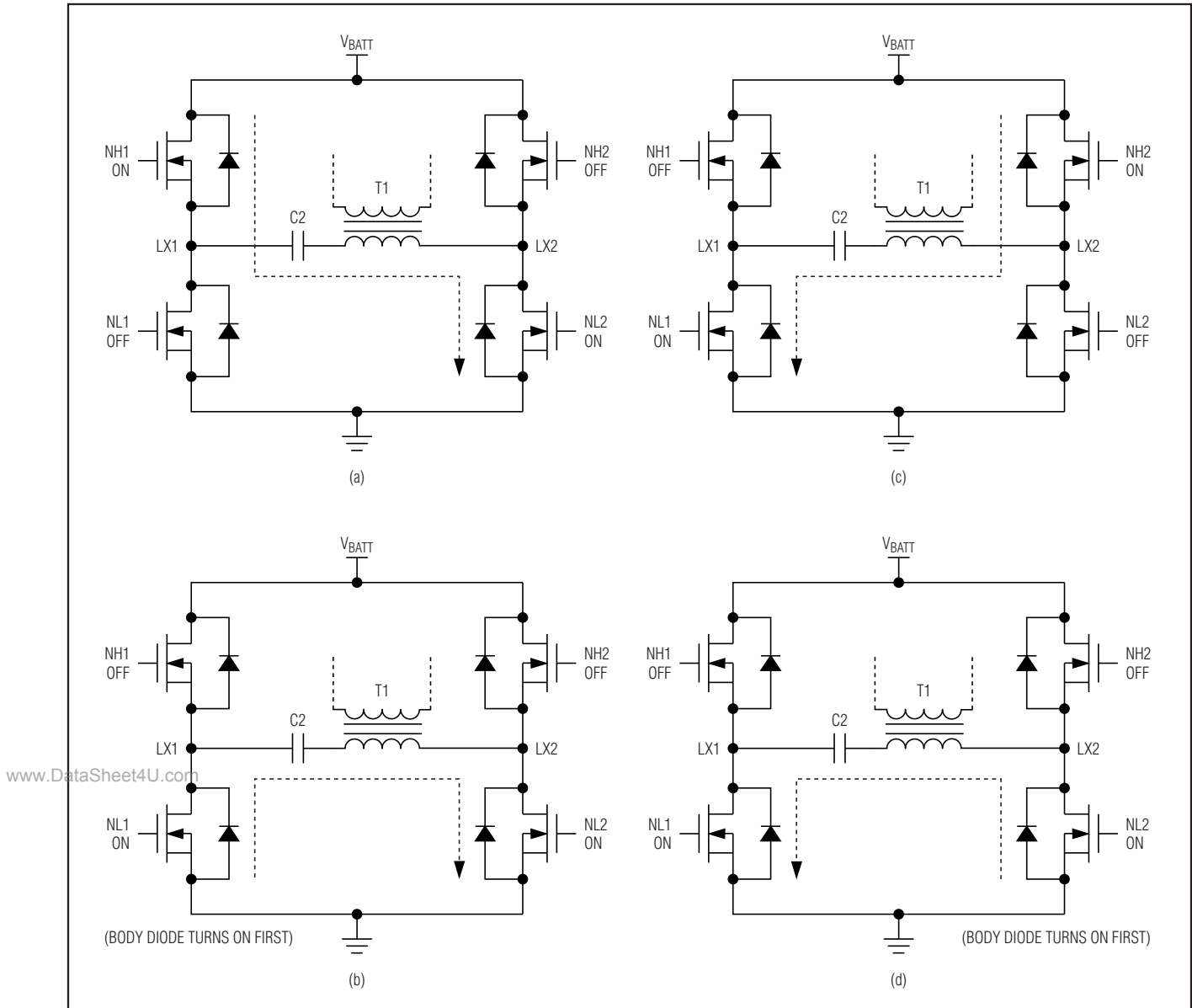
Figure 3. Resonant Operation
