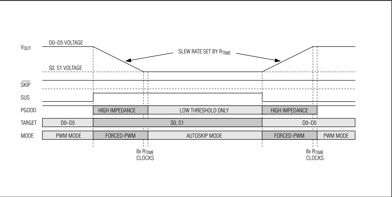
Figure 10. Suspend Transition in Forced-PWM Mode ( \overline{\text{SKIP}} = \text{High} )
