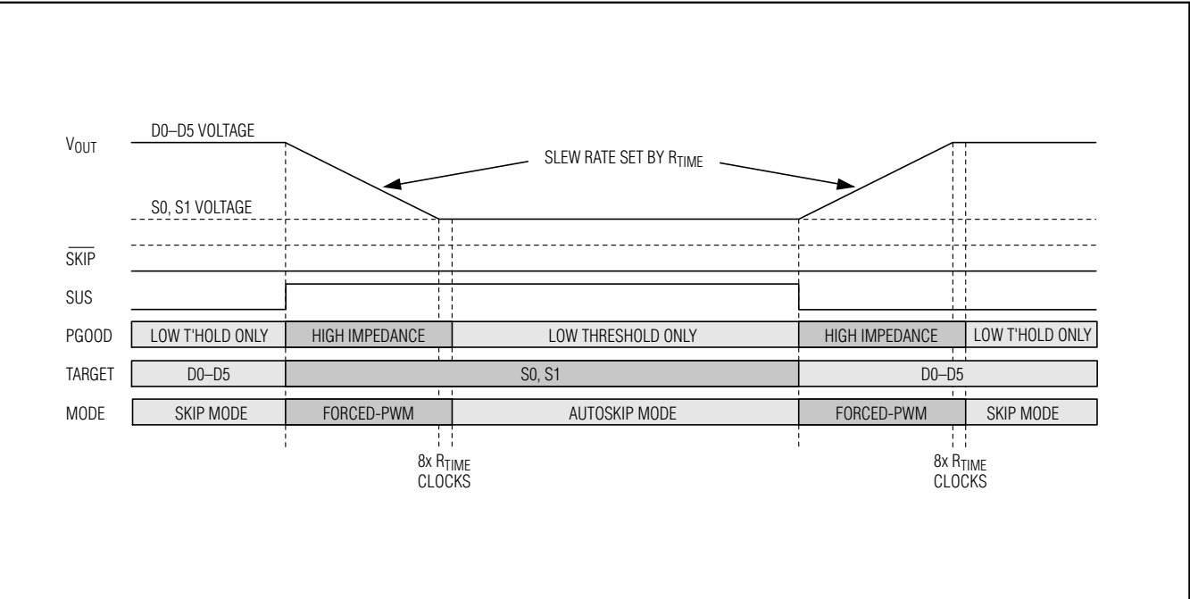
Figure 11. Suspend Transition in Pulse-Skipping Mode ( \overline{\text{SKIP}} = \text{GND} )
