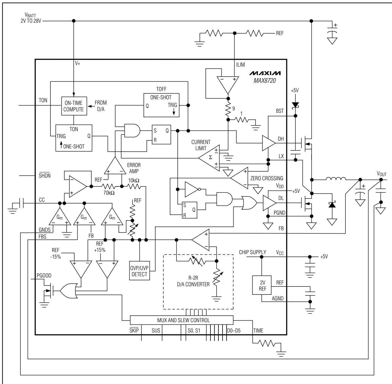
Figure 2. MAX8720 Block Diagram
