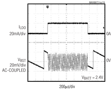
BST RESPONSE TO LDO LOAD TRANSIENT
