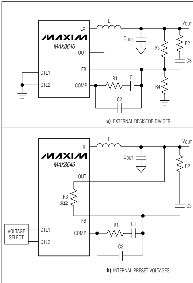
Figure 3. Type III Compensation Network
