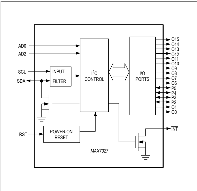
Functional Diagram
