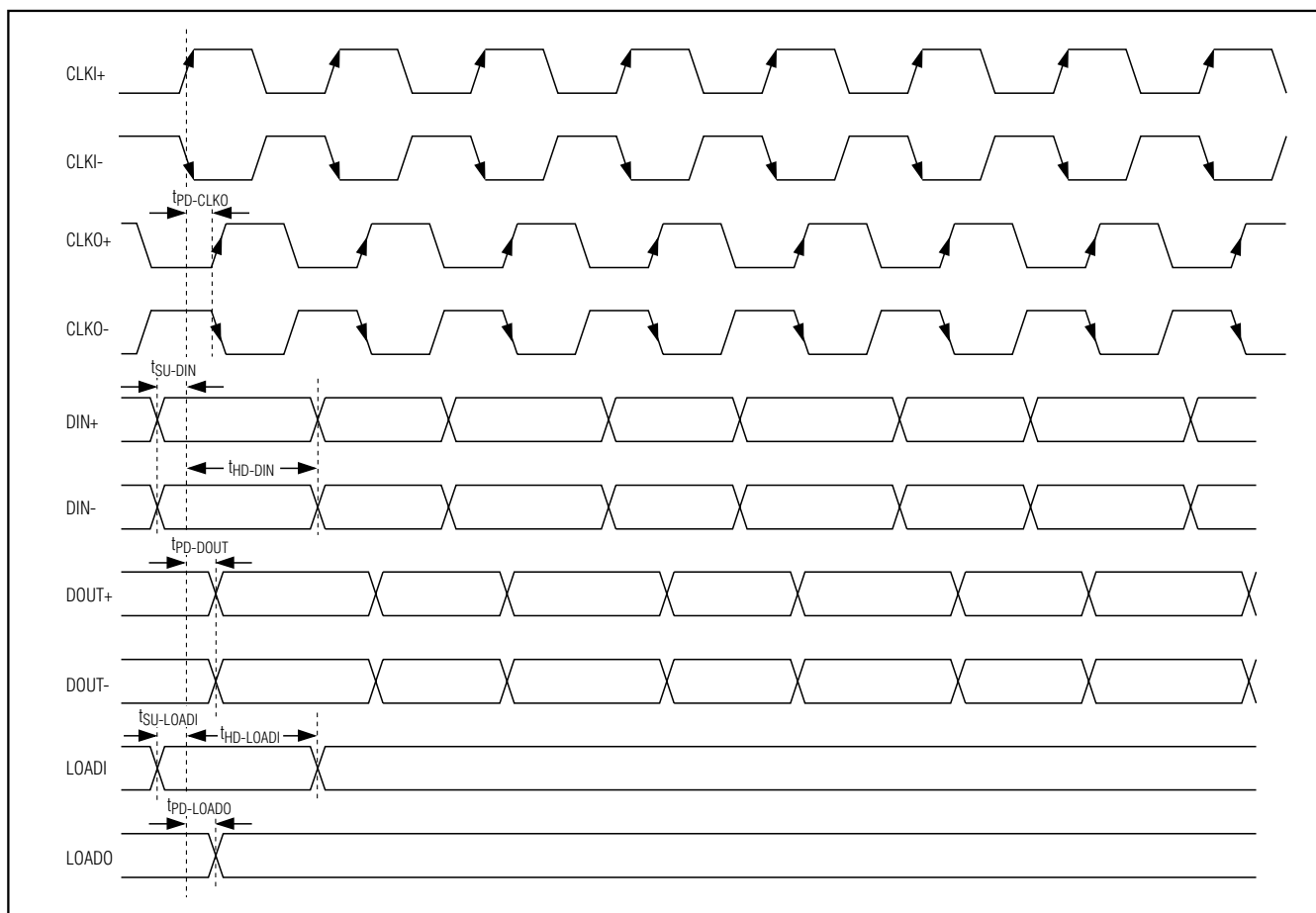
Figure 6. Serial-Interface Timing
