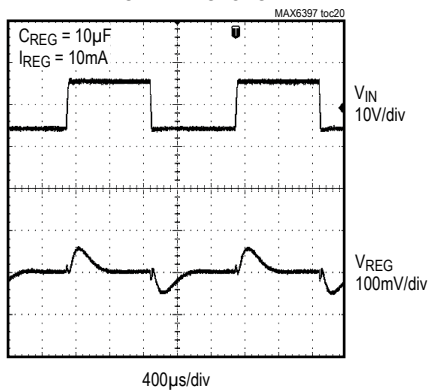
TRANSIENT RESPONSE
