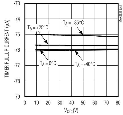
MAX5947_ TIMER PULLUP CURRENT vs. V_{CC}
