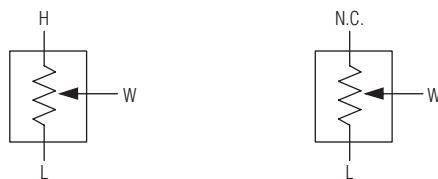
Figure 1. Voltage-Divider and Variable Resistor Configurations
