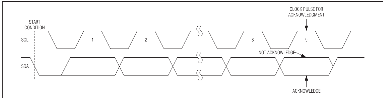
Figure 6. Acknowledge
