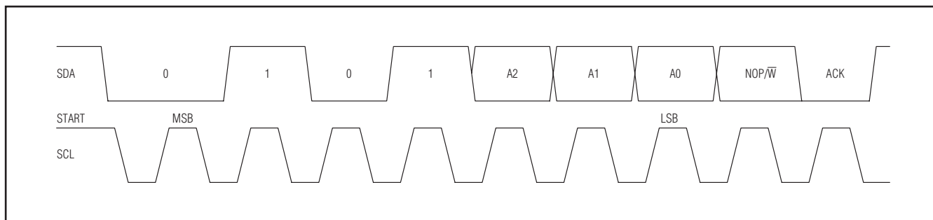
Figure 4. Slave Address
