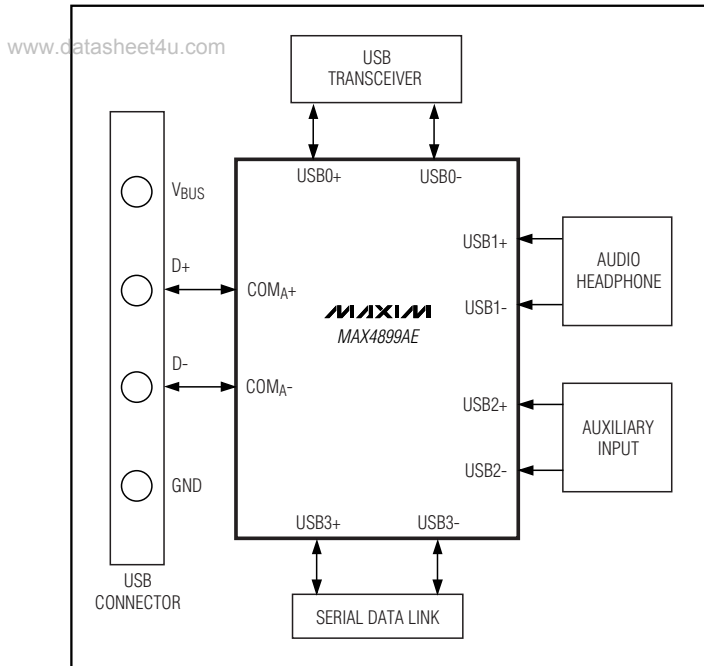
Figure 8. MAX4899AE Multiplexing Four Data Types
