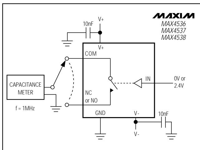
Figure 6. Channel-Off Capacitance
