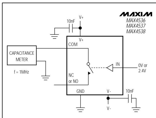
Figure 7. Channel-On Capacitance
