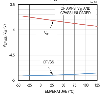
CPVSS AND V_{SS} vs. TEMPERATURE ( V_{DD} = 5\text{V} )
