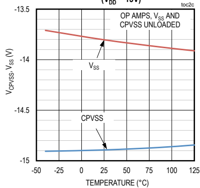
CPVSS AND V_{SS} vs. TEMPERATURE ( V_{DD} = 15\text{V} )
