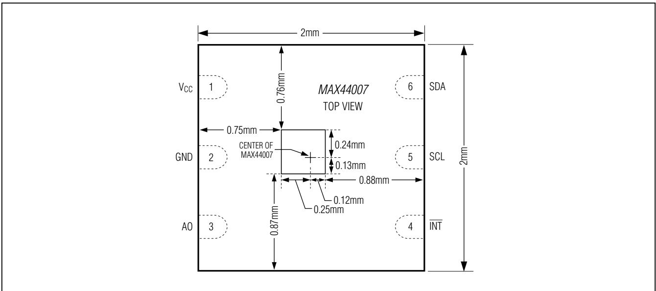
Figure 8. Sensor Position
