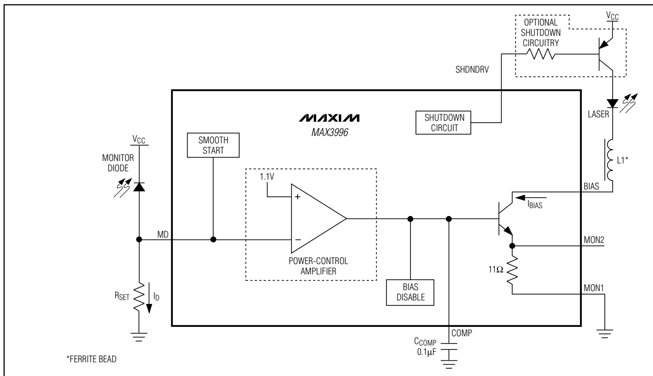
Figure 11. APC Loop
