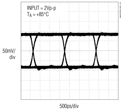
DATA OUTPUT SINGLE-ENDED (2 23 -1 PRBS PATTERN)
