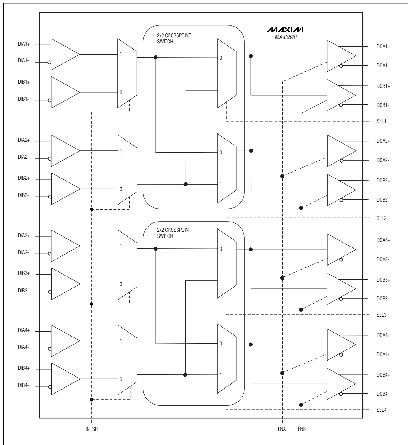
Figure 2. Functional Diagram
