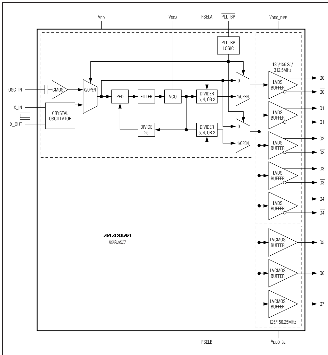
Figure 3. Functional Diagram
