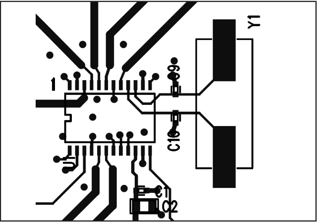
Figure 2. Crystal Layout
