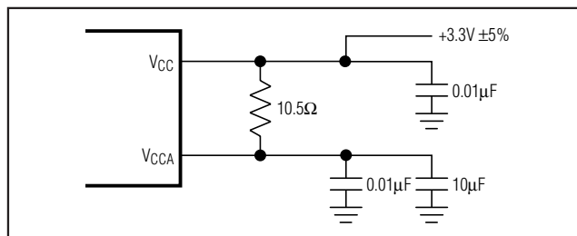
Figure 1. Analog Supply Filtering
