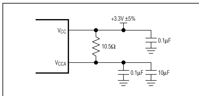
Figure 2. Analog Supply Filtering
