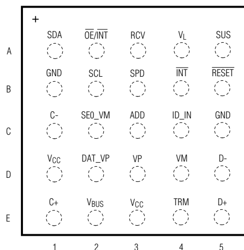
WLP PACKAGE (2.54mm x 2.54mm)
