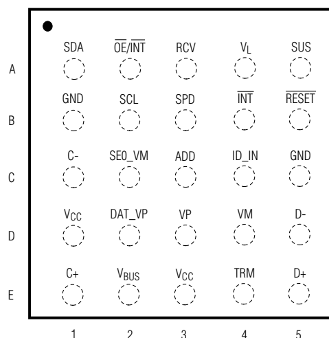
UCSP (2.5mm x 2.5mm)
