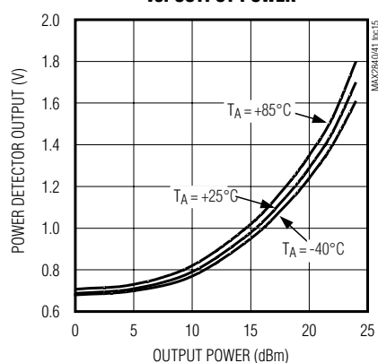
MAX2841 POWER DETECTOR OUTPUT vs. OUTPUT POWER
