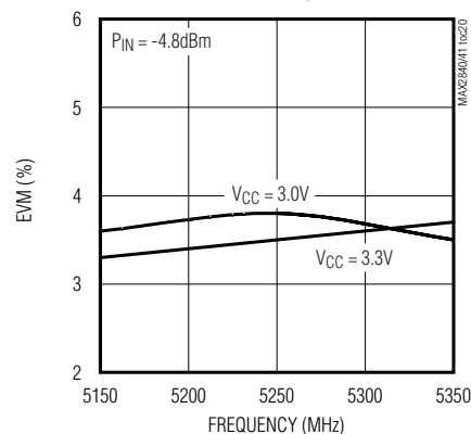
MAX2841 EVM vs. FREQUENCY
