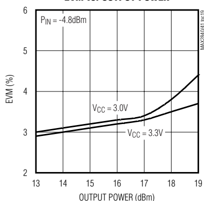
MAX2841 EVM vs. OUTPUT POWER
