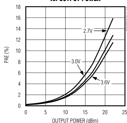
MAX2841 POWER-ADDED EFFICIENCY (PAE) vs. OUTPUT POWER
