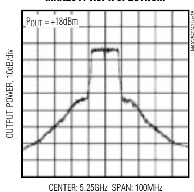
MAX2841 ACPR SPECTRUM
