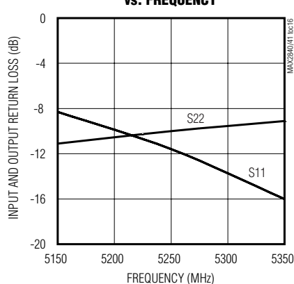
MAX2841 INPUT AND OUTPUT RETURN LOSS vs. FREQUENCY
