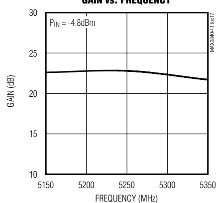
MAX2841 GAIN vs. FREQUENCY
