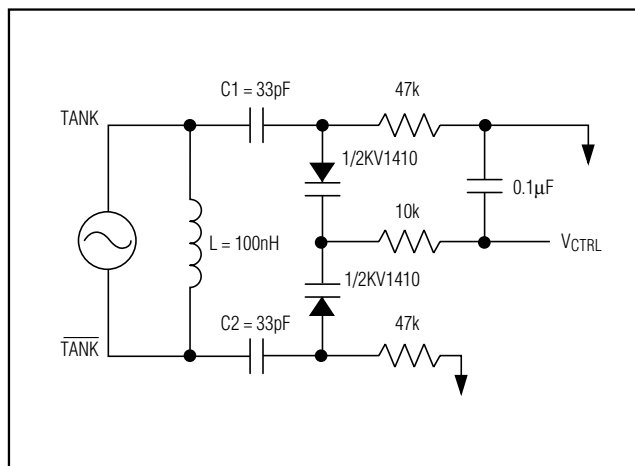
Figure 3. Typical Resonant Tank Circuit
