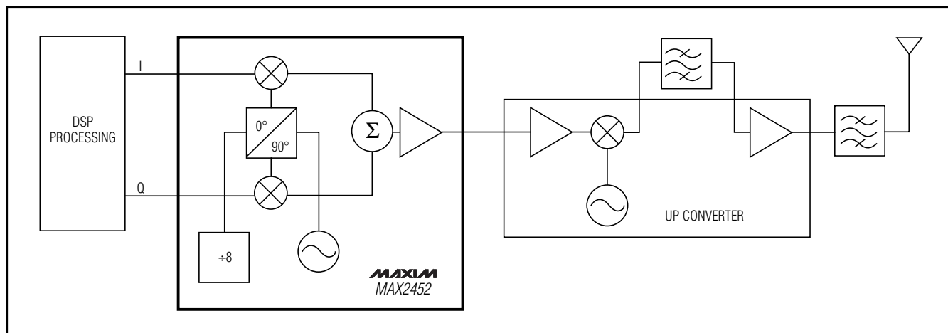
Figure 2. Typical Application Block Diagram
