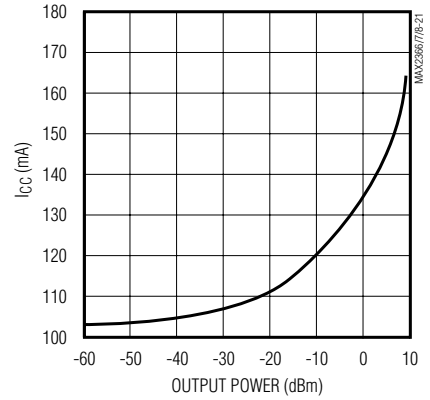
I_{CC} vs. RFH1 OUTPUT POWER (1880MHz)
