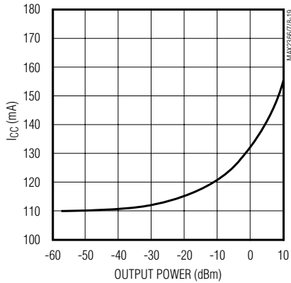
I_{CC} vs. RFL OUTPUT POWER (836MHz)
