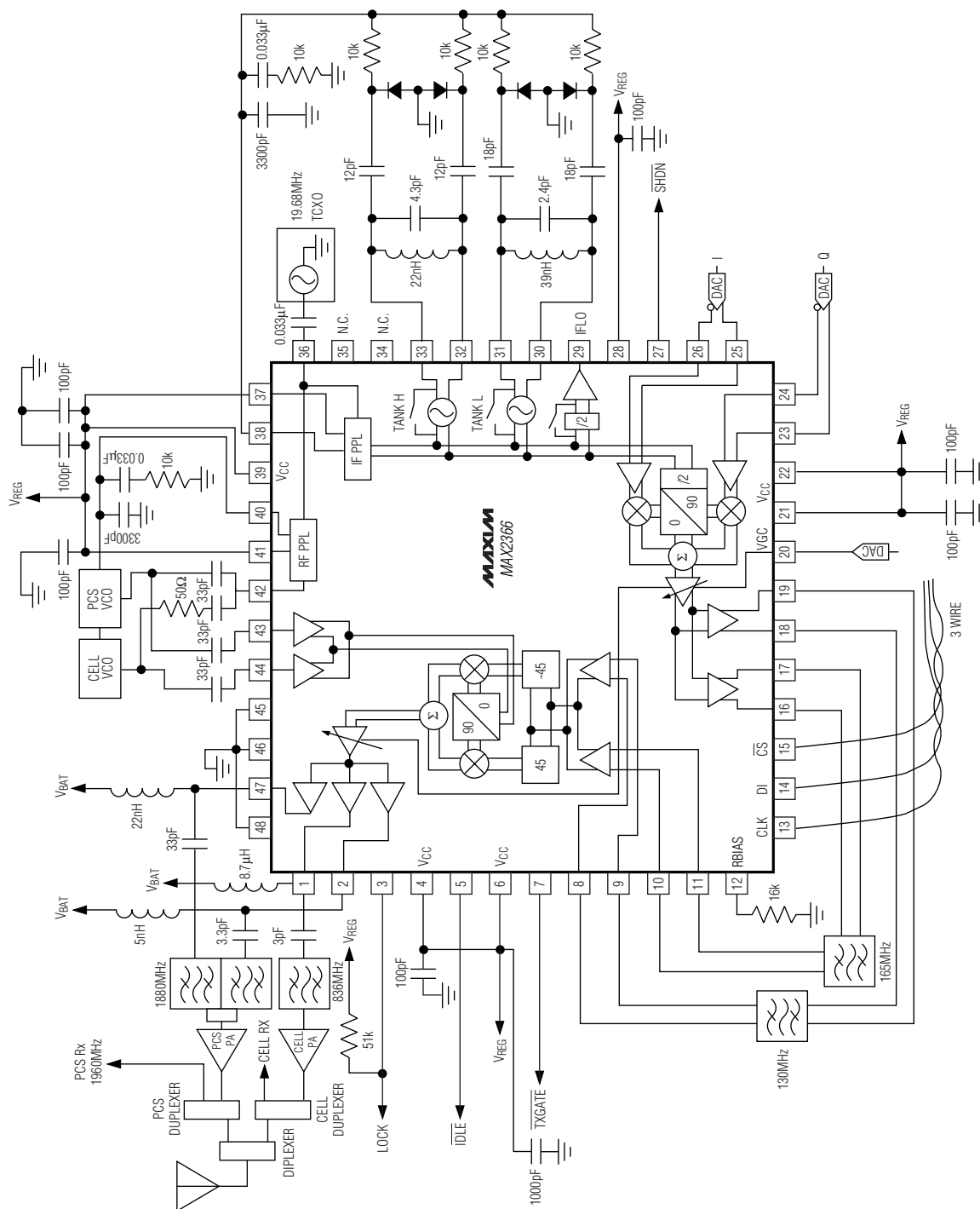
Figure 2. MAX2366 Typical Application Circuit
