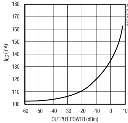
I_{CC} vs. RFH0 OUTPUT POWER (1880MHz)
