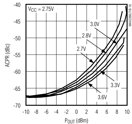
CASCADE ACPR vs. P OUT AND V BAT
