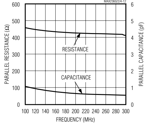
IF/IN DIFFERENTIAL PORT INPUT IMPEDANCE
