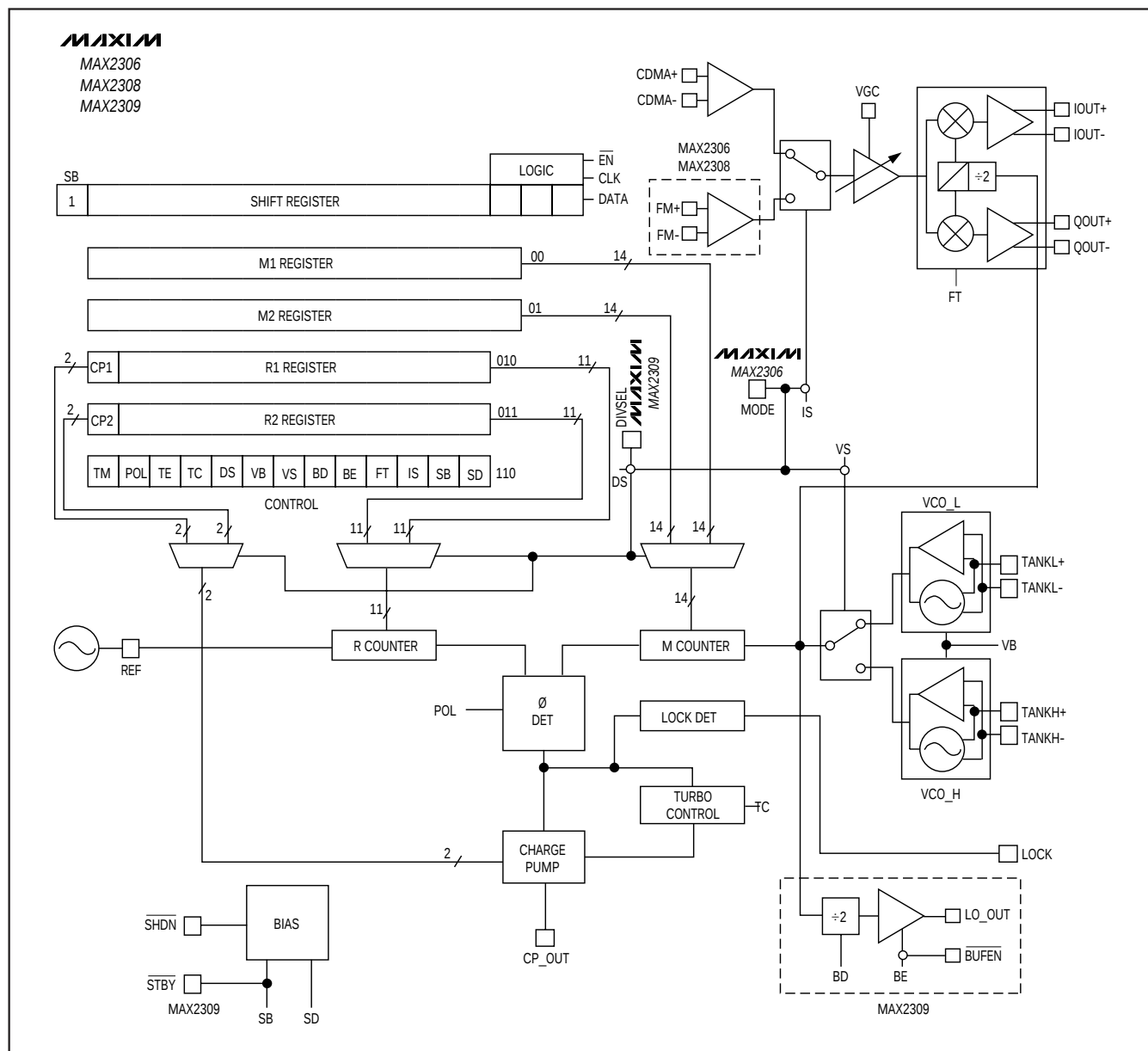
Functional Diagram
