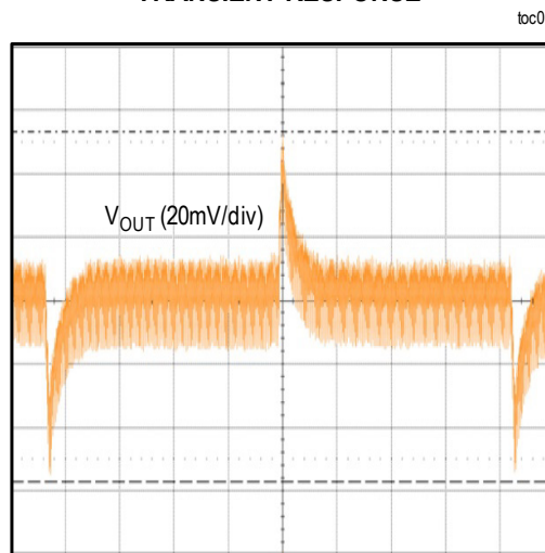
TRANSIENT RESPONSE
