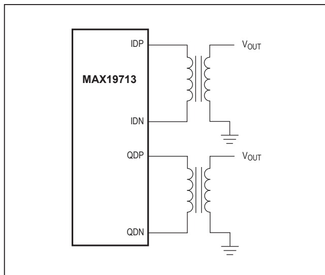
Figure 10. Balun Transformer-Coupled Differential-to-Single-Ended Output Drive for Tx DAC
