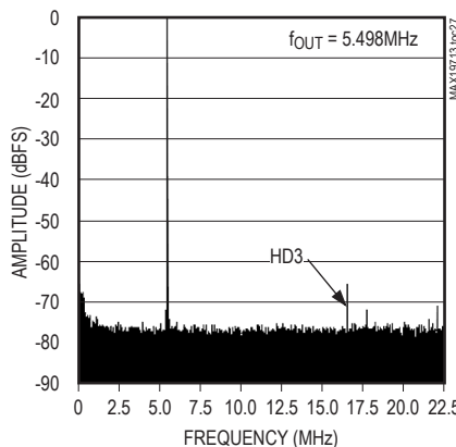
Tx DAC CHANNEL-QD SPECTRAL PLOT
