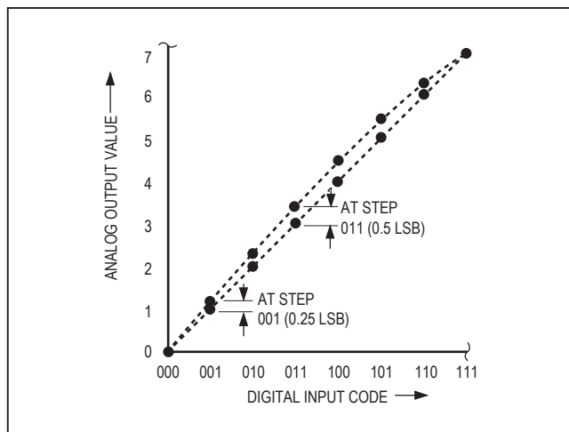
Figure 14a. Integral Nonlinearity
