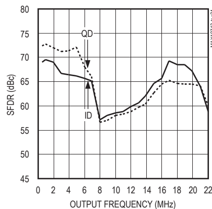
Tx DAC SPURIOUS-FREE DYNAMIC RANGE vs. OUTPUT FREQUENCY
