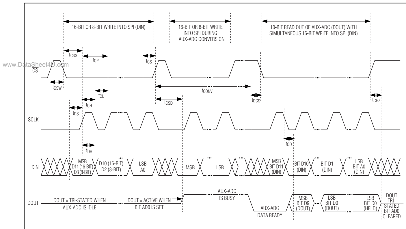
Figure 6. Serial-Interface Timing Diagram
