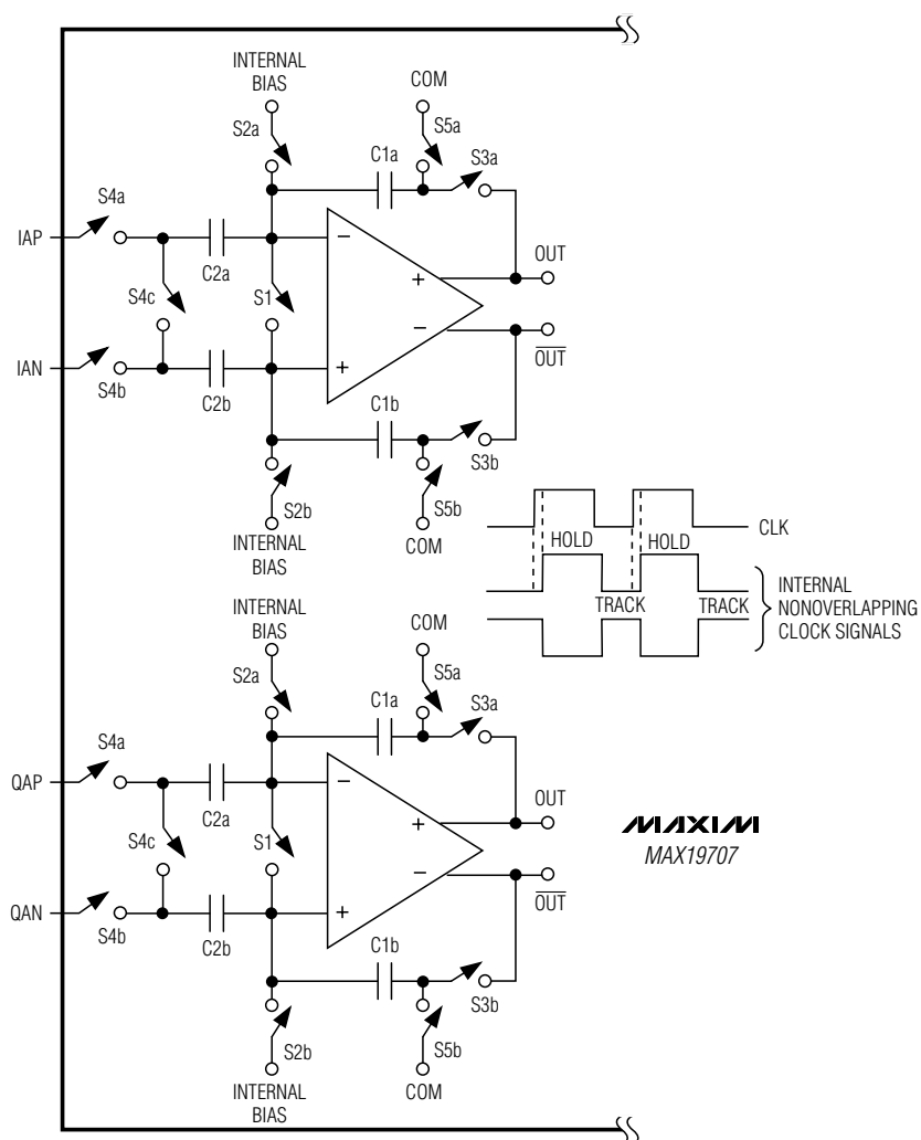
Figure 1. Rx ADC Internal T/H Circuits
