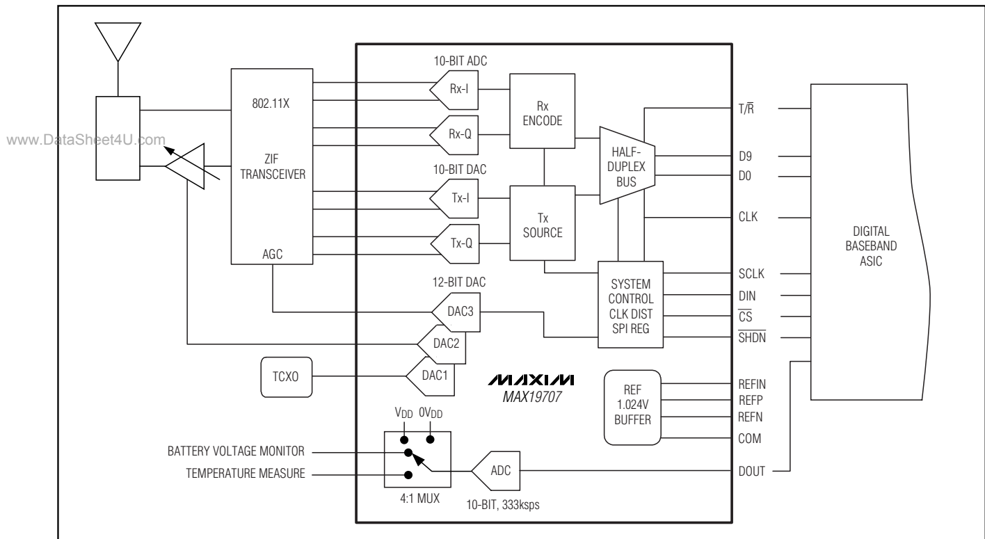
Figure 12. Typical Application Circuit for 802.11 Radio
