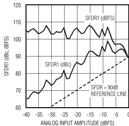
SFDR1 vs. ANALOG INPUT AMPLITUDE ( f_{CLK} = 80MHz , f_{IN} = 10.10011MHz )
