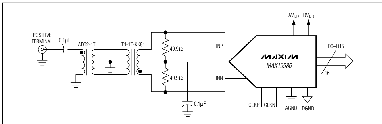
Figure 7. Transformer-Coupled Analog Input Configuration with Primary-Side Balun Transformer
