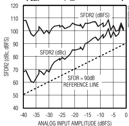
SFDR2 vs. ANALOG INPUT AMPLITUDE ( f_{CLK} = 80MHz , f_{IN} = 70.163683MHz )
