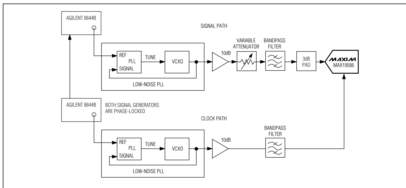
Figure 8d. Improved Test System Employing Narrowband PLLs (Simplified Block Diagram)
