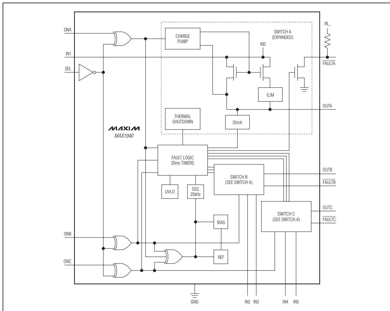
Figure 1. Functional Diagram
