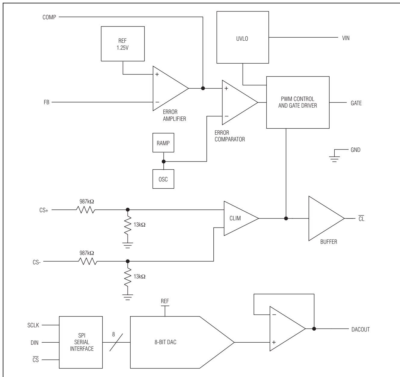
Figure 1. Functional Diagram
