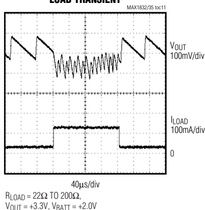
LOAD TRANSIENT
