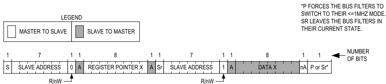
Figure 10. Reading from a Single Register with the Read Byte Protocol
