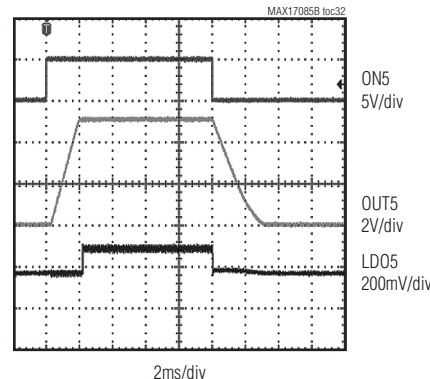
SMPS5 STARTUP AND SHUTDOWN LOAD
