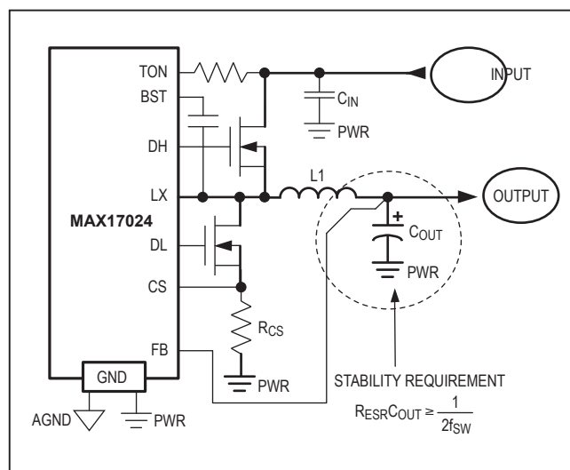
Figure 6. Standard Application with Output Polymer or Tantalum
