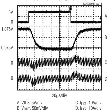
DYNAMIC VID CODE CHANGE ( D0 = 12.5mV )
