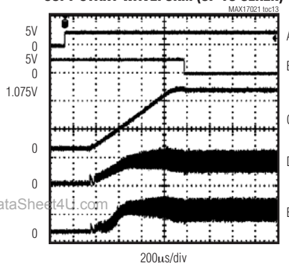
SOFT-START WAVEFORM (UP TO CLKEN)
