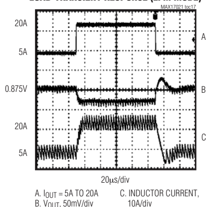
LOAD-TRANSIENT RESPONSE (LFM MODE)
