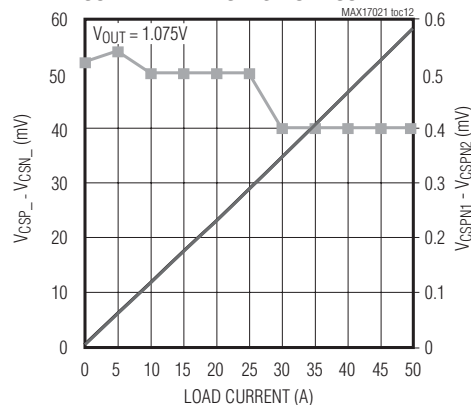
CURRENT BALANCE vs. LOAD CURRENT
