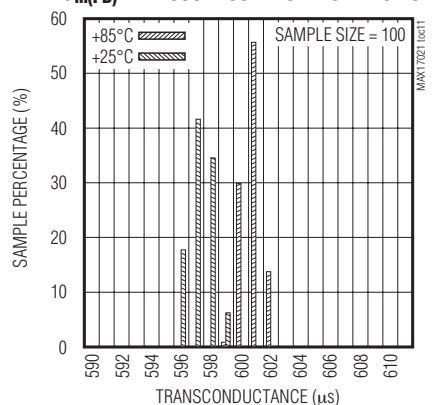
G_m(FB) TRANSCONDUCTANCE DISTRIBUTION
